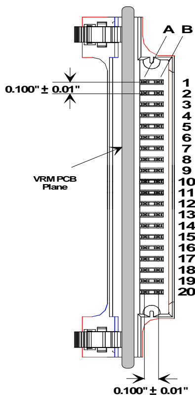
Figure 2, Pin Orientation
